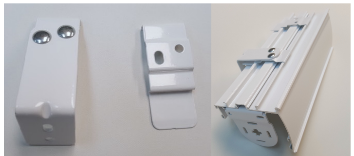
Face fit bracket (L) for fixing pelmet to the wall and top fix bracket (R) for fixing pelmet to the ceiling.
